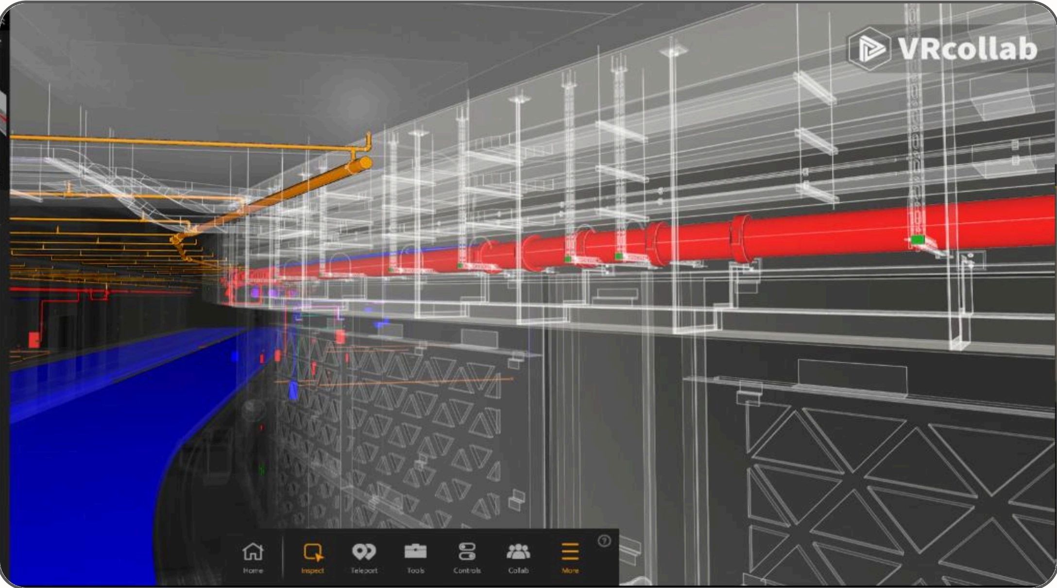
DGCL North & South Main Spine Tunnel Wireframe View of Tunnel in VR Collab
